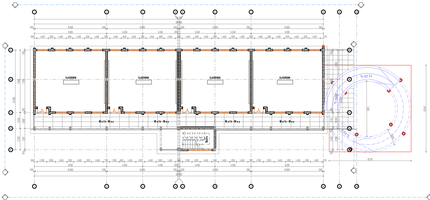
FIRST FLOOR PLAN SCALE 1:200
