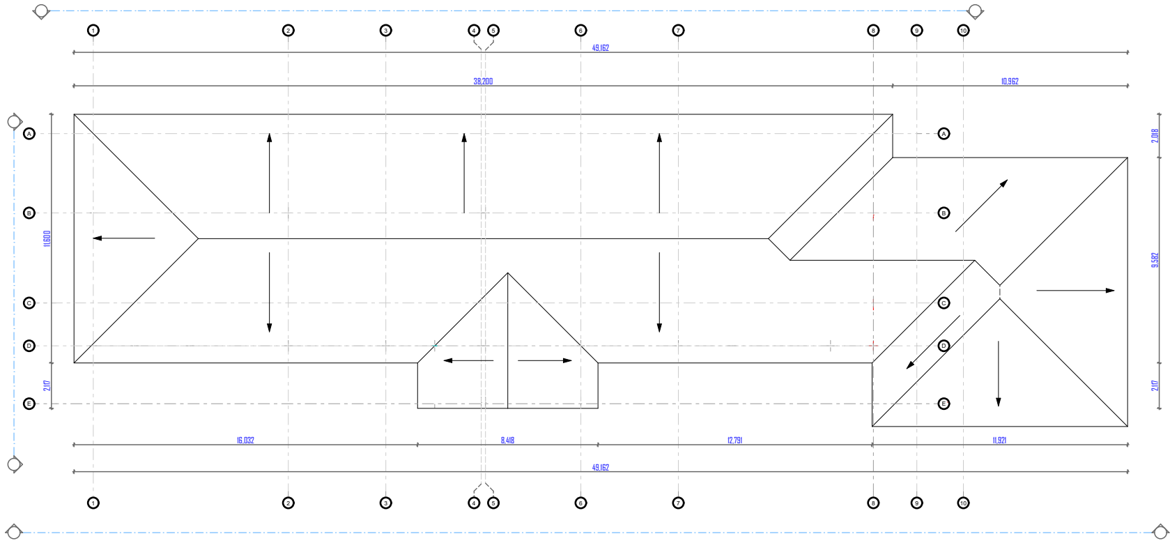
ROOF LAYOUT PLAN SCALE 1:200
