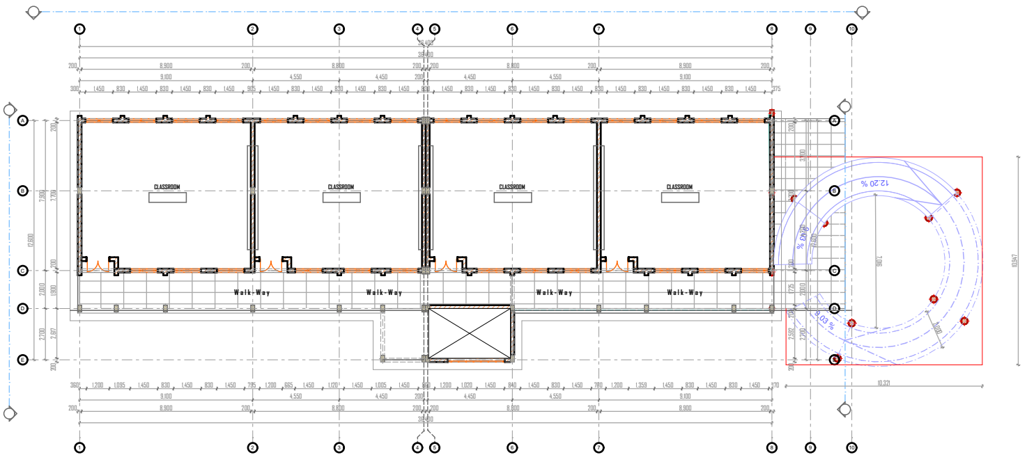
SECOND FLOOR PLAN SCALE 1:200
